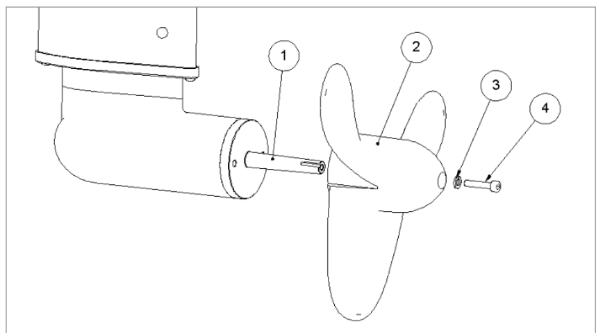
[Figure 11] Components required for installing the turbine:
