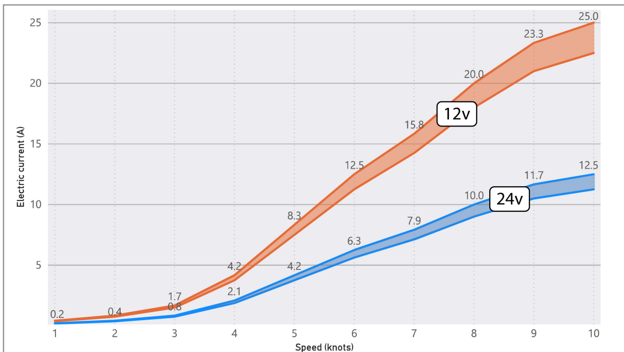
[Figure 35] Charging current at different operating speeds
