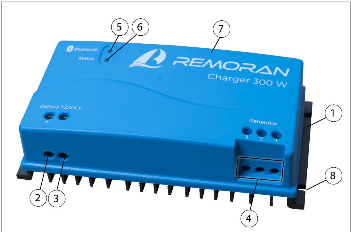
[Figure 3] CHARGER COMPONENTS:
